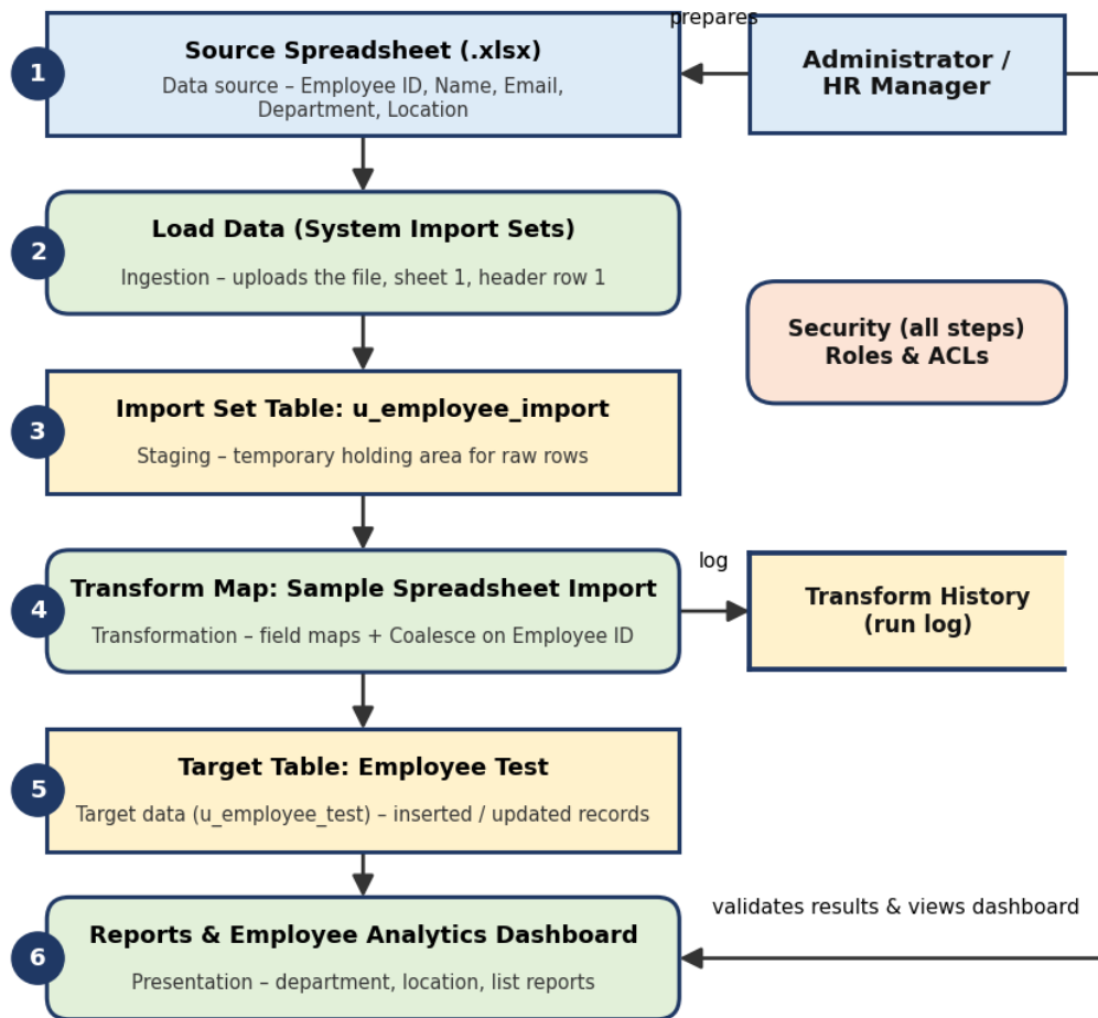
Figure 1: Architecture and data flow of the employee data import solution
